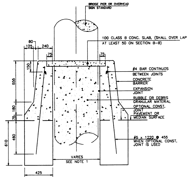
SECTION B-B
