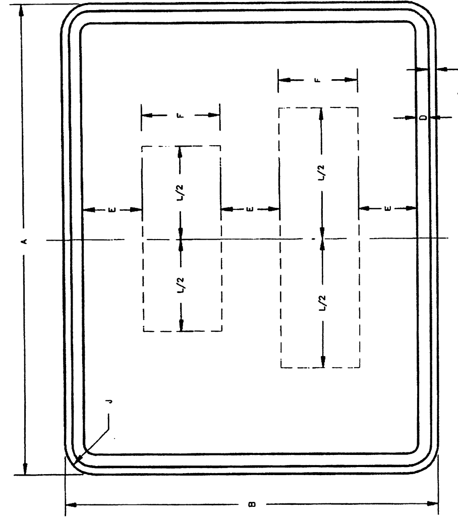
PARADOR AND MESON NAME PLATE DOUBLE LINE TEXT RM-53
