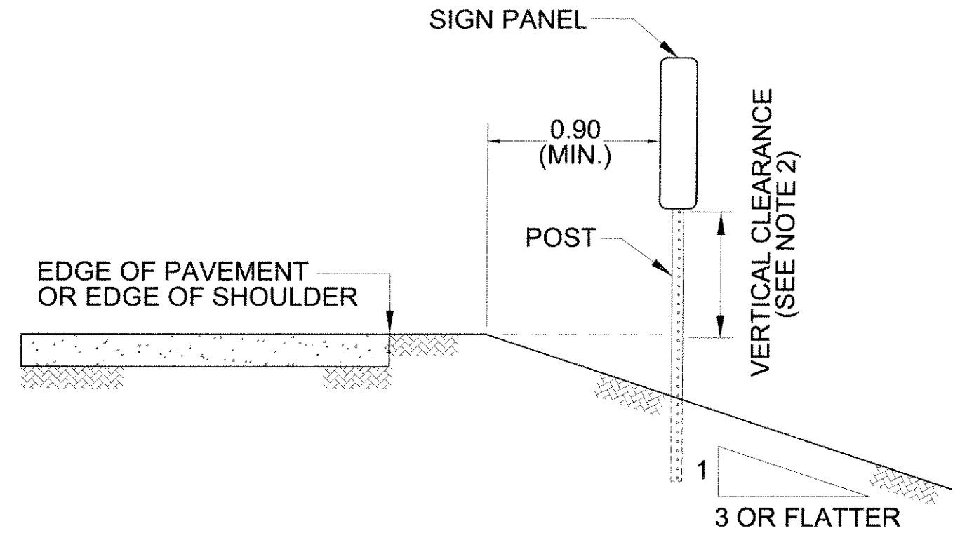
EMBANKMENTS WITH SLOPES 3:1 OR FLATTER
