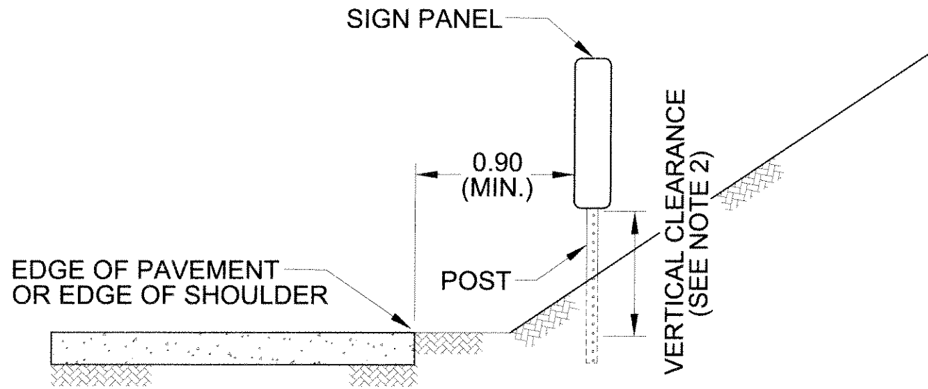
CUT SECTIONS
