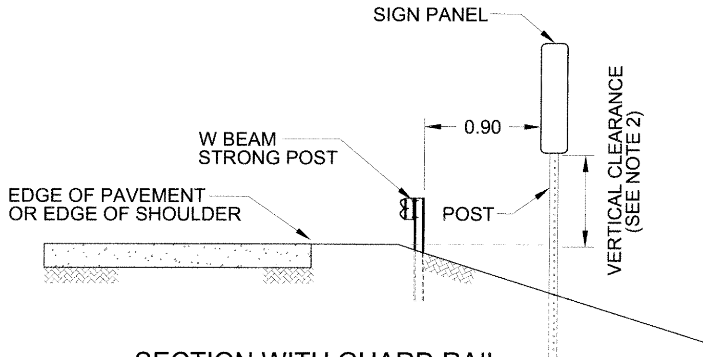
SECTION WITH GUARD RAIL
